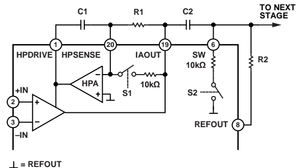
Figure 54. Schematic for a Two-Pole High-Pass Filter
