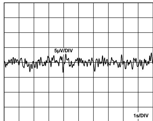
Figure 26. Operational Amplifier 0.1 Hz to 10 Hz Noise
