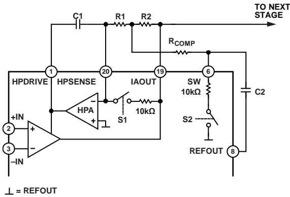
Figure 55. Schematic for an Alternative Two-Pole High-Pass Filter
