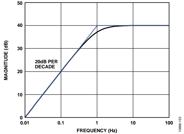
Figure 53. Frequency Response of Single-Pole DC Blocking Circuit
