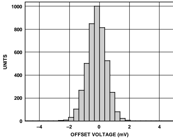
Figure 21. Operational Amplifier Offset Distribution
