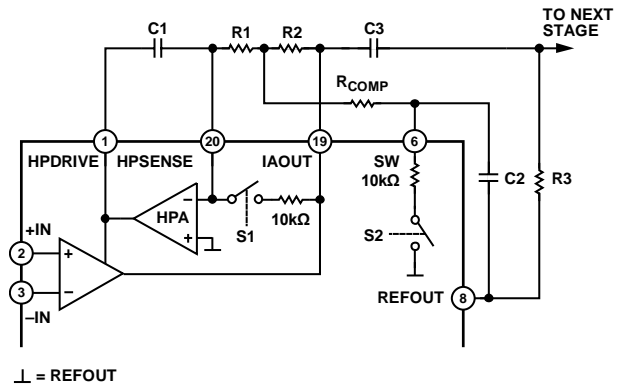
Figure 56. Schematic for a Three-Pole High-Pass Filter
