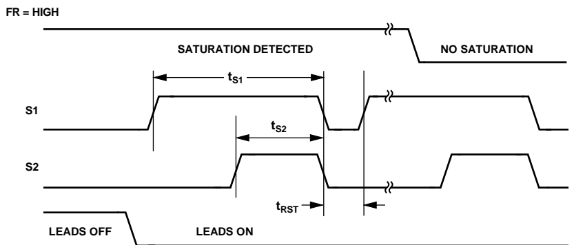
Figure 48. Timing Diagram for Fast Restore Switches (Time Base Not to Scale)
