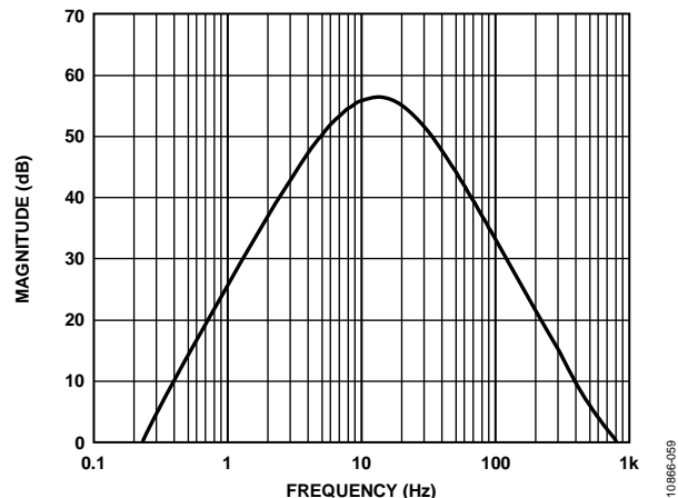
Figure 63. Frequency Response for HRM Circuit Taken at the Hands
