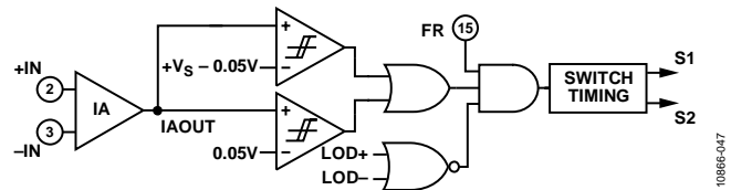
Figure 47. Fast Restore Circuit
