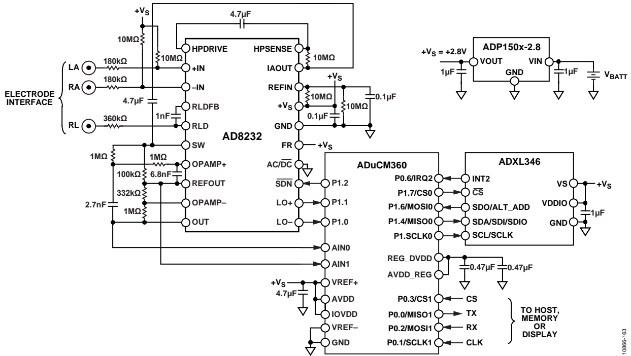
Figure 66. Low Power Portable Cardiac Monitor
