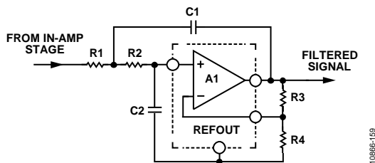
Figure 59. Schematic for a Two-Pole Low-Pass Filter
