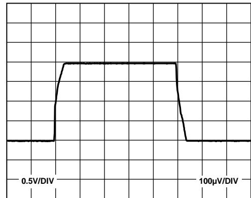
Figure 24. Operational Amplifier Large Signal Transient Response
