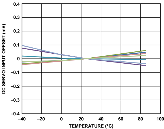
Figure 17. Instrumentation Amplifier DC Blocking Input Offset Drift
