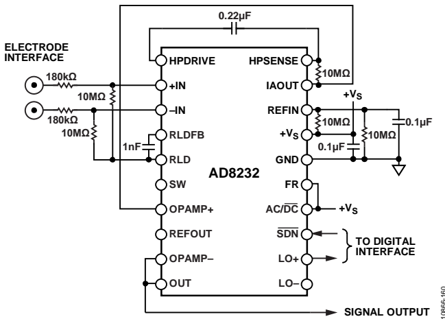
Figure 60. Circuit for Heart Rate Measurement Next to Heart
