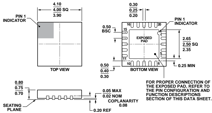
Figure 67. 20-Lead Lead Frame Chip Scale Package [LFCSP_WQ] 4 mm × 4 mm Body, Very Very Thin Quad (CP-20-10) Dimensions shown in millimeters
