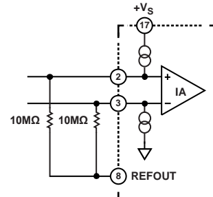
Figure 50. Circuit Configuration for AC Leads Off Detection
