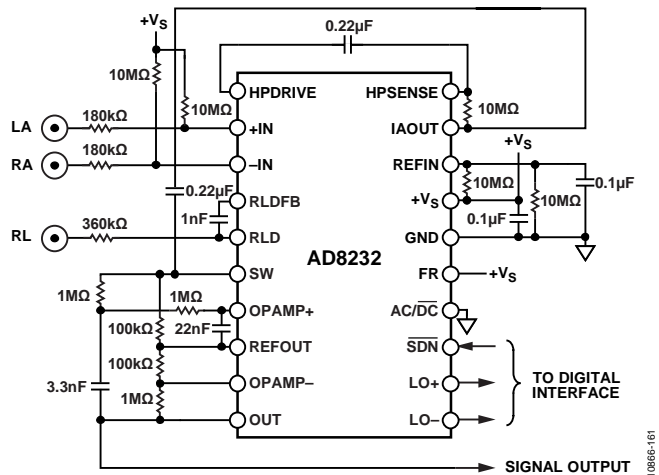
Figure 62. Circuit for Heart Rate Measurement at Hands
