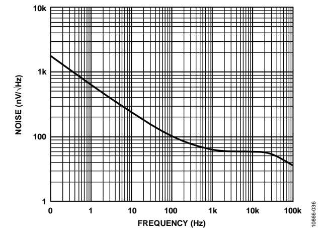
Figure 36. RLD Amplifier Voltage Spectral Noise Density vs. Frequency
