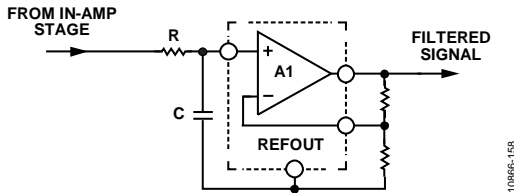
Figure 58. Schematic for a Single-Pole Low-Pass Filter and Additional Gain
