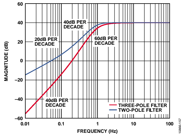
Figure 57. Frequency Response of Circuits in Figure 55 and Figure 56
