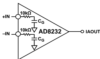
Figure 51. RFI Filter Without External Capacitors
