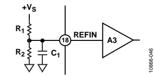
Figure 46. Setting the Internal Reference
