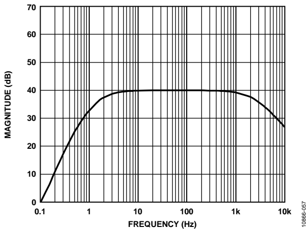
Figure 61. Frequency Response for HRM Next to Heart Circuit
