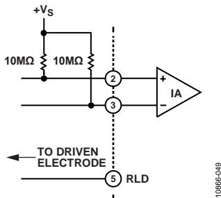
Figure 49. Circuit Configuration for DC Leads Off Detection
